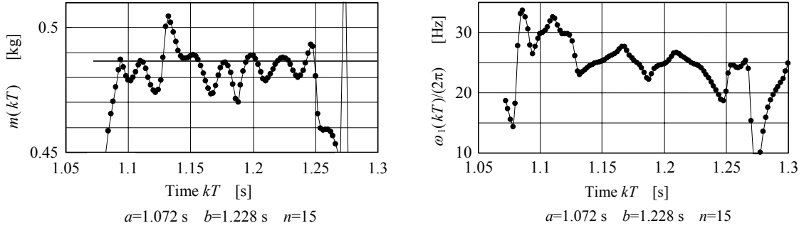
Fig. 6. Estimated values obtained by using G_i(z) designed for f(kT) in Fig. 5; a) the estimated mass of object m(kT) and b) the estimated angular frequency of dominant component \omega_1(kT)/(2\pi) .
